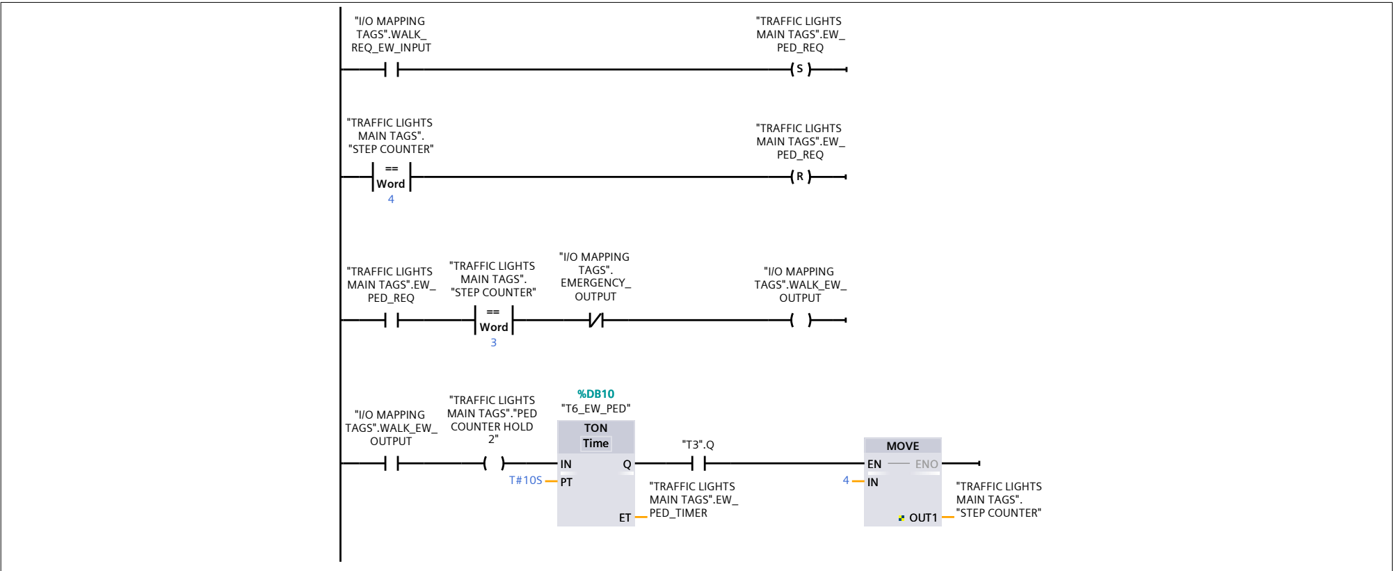
Network 8: EMERGENCY CONDITION
